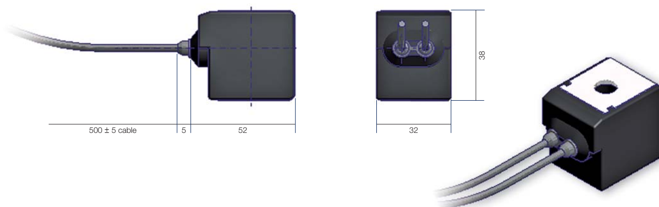
Dimensional Drawing N° 28
