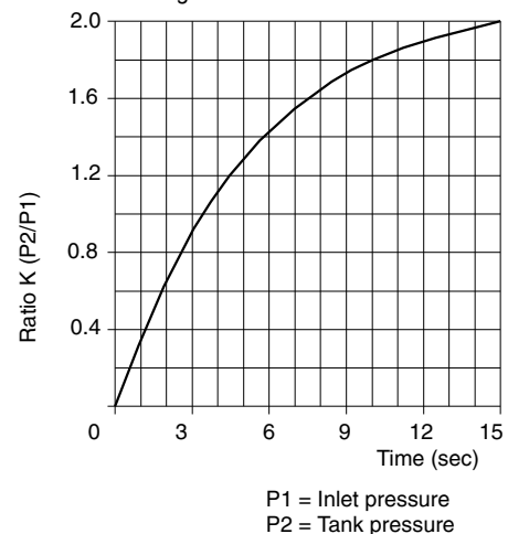
Filling time curve of 10 liters tank
